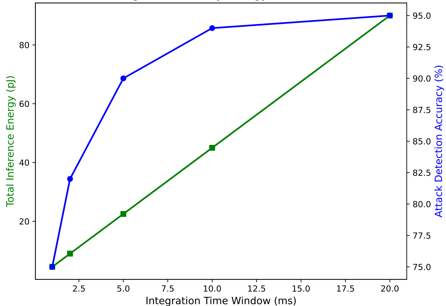
Figure 7: Latency-Energy Tradeoff
